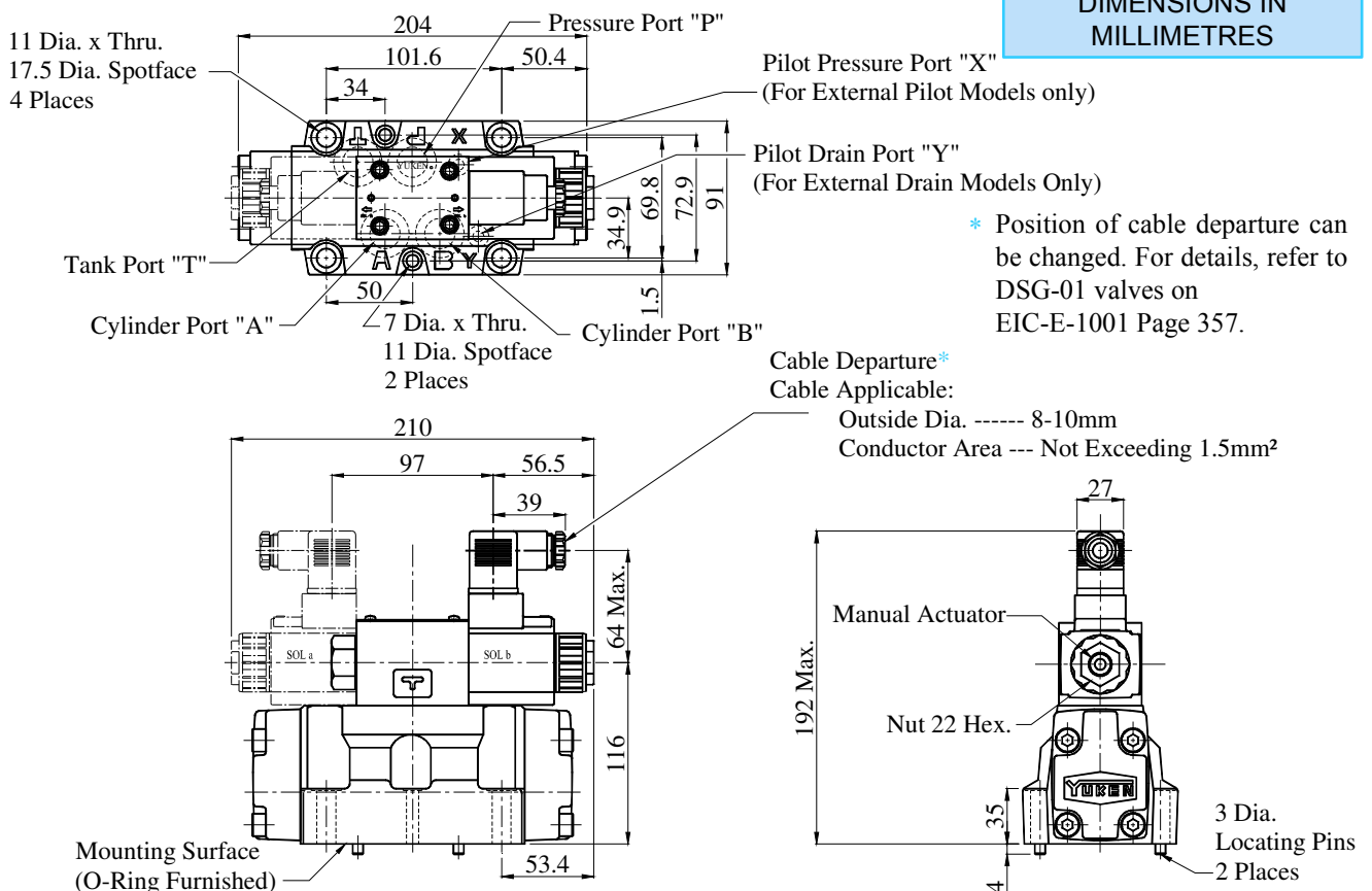
Solenoid Controlled Pilot Operated Directional Valves
