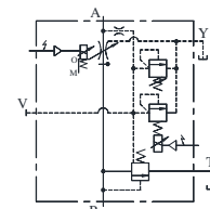
Models With Proportional Pilot Relief Valve
