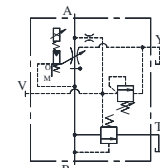
Models With Proportional Pilot Relief Valve
