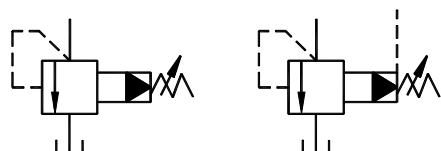
Vent Connection
