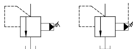
Vent Connection
